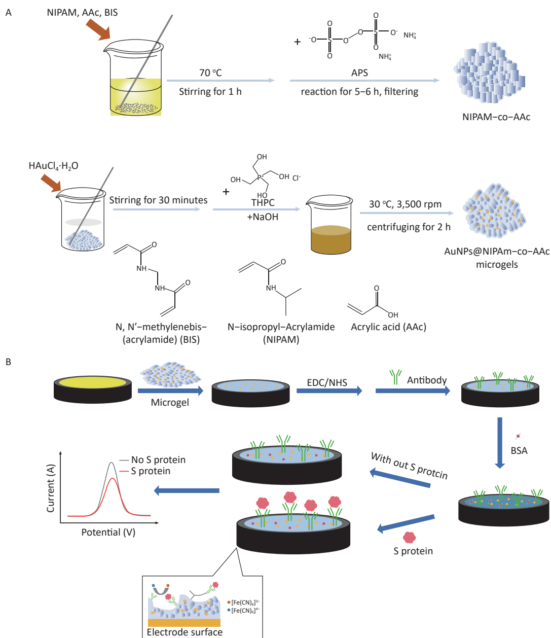
Supplementary Figure S1. (A) Synthesis of AuNPs@NIPAM-co-AAc microgels. (B) Construction of the sensing platform and detection process of S protein.
