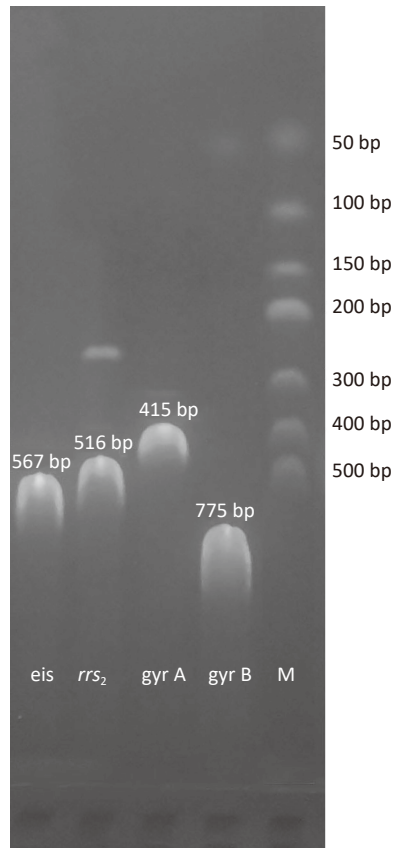
Supplementary Figure S1. Agarose gel electrophoresis of PCR assays for the identification of eis , rrs 2 , gyrA , and gyrB genes. M: DL500 DNA Marker (Takara, Code No. 3590A).
