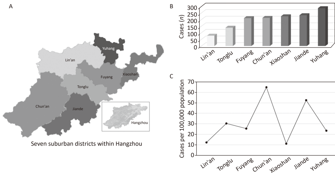
Supplementary Figure S2. The spatial distributions and TB prevalence rate of seven districts in Hangzhou from 2019 to 2020. Spatial distributions of seven suburban districts within Hangzhou (A); Distributions of TB incidences ( n ) (B); Incidences of TB cases per 100,000 population by districts (C).
