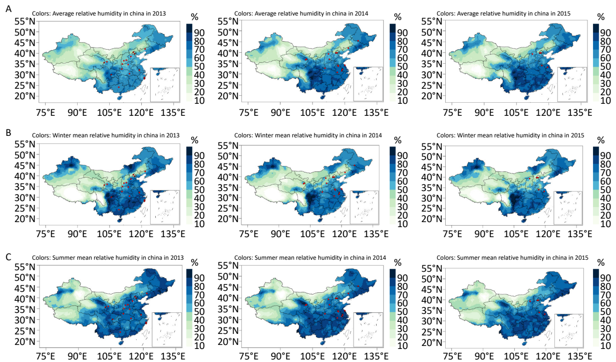
Supplementary Figure S1. Average annual relative humidity (A), winter mean relative humidity (B), and summer mean relative humidity (C) in China, 2013–2015. Red dots denote survey sites in the baseline year.
