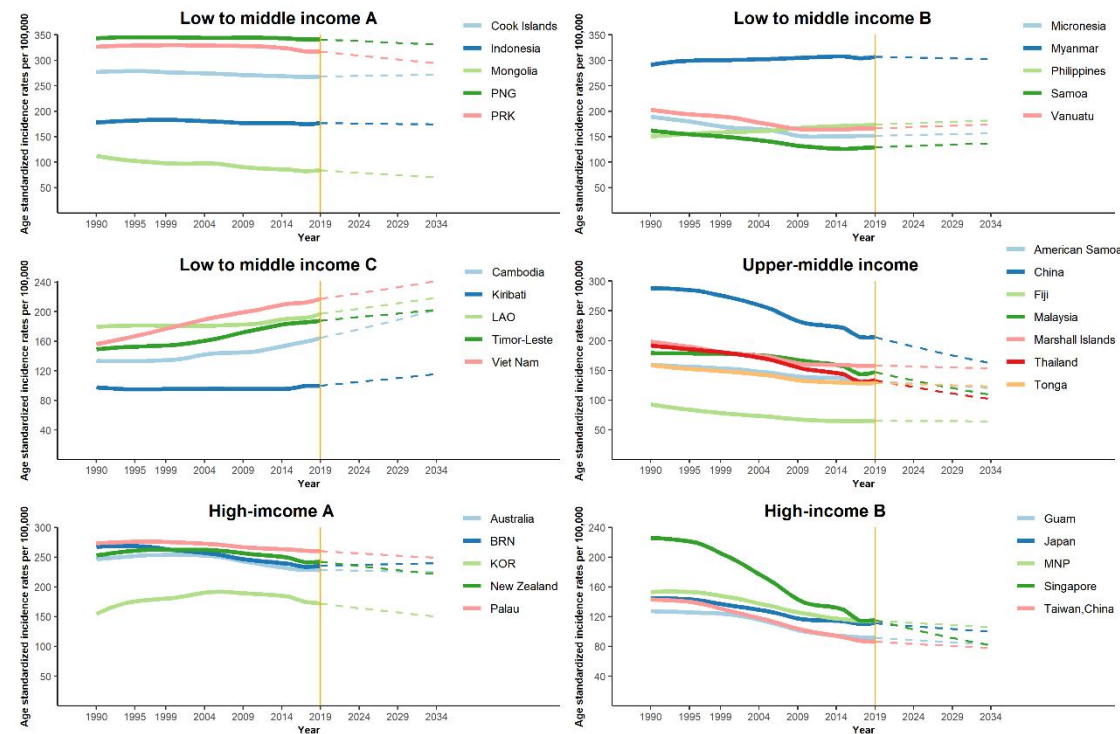
Supplementary Figure S2. Trends in observed (solid lines) and predicted (dashed lines) COPD incidence rates in selected Asia-Pacific countries and territories, 1990-2034. PNG means Papua New Guinea, PRK means Democratic People's Republic of Korea, Micronesia means Micronesia (Federated States of), LAO means Lao People's Democratic Republic, BRN means Brunei Darussalam, KOR means Republic of Korea, MNP means Northern Mariana Islands.
