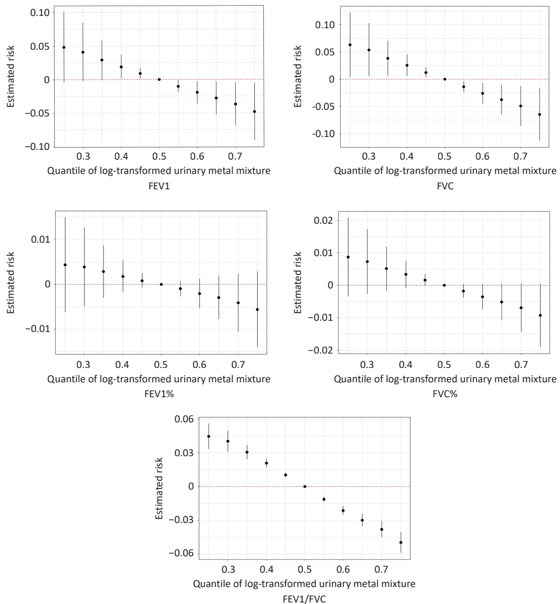
Figure 1. BKMR assesses the overall association between metal-mixture exposure and lung function indicators. The figure shows the estimated total effects of combined exposure to six metals at specific percentiles on lung function indicators and their 95% confidence intervals. The model was adjusted for age, BMI, smoking, drinking, occupational dust, years of work, education, and exercise. FEV_1 , forced expiratory volume in the first second; FEV_1\% , percentage of predicted forced expiratory volume in the first second; FVC, forced vital capacity; FVC%, percentage of predicted forced vital capacity; FEV_1/FVC , ratio of forced expiratory volume in the first second to forced vital capacity; BMI, body mass index.
